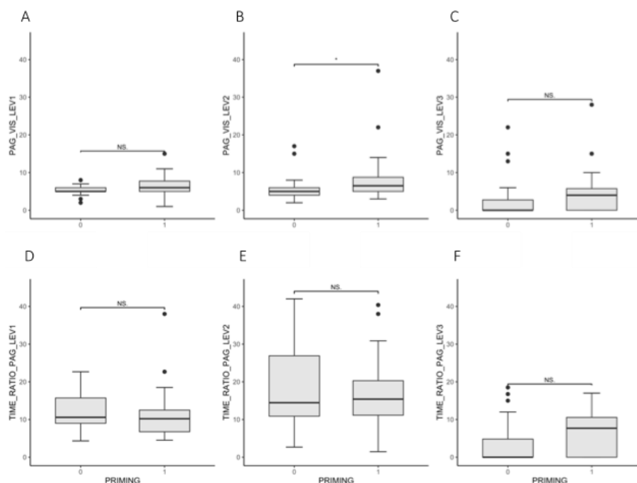
Figure 4. Boxplot for H 3 to H 8 (Mann-Whitney test)
