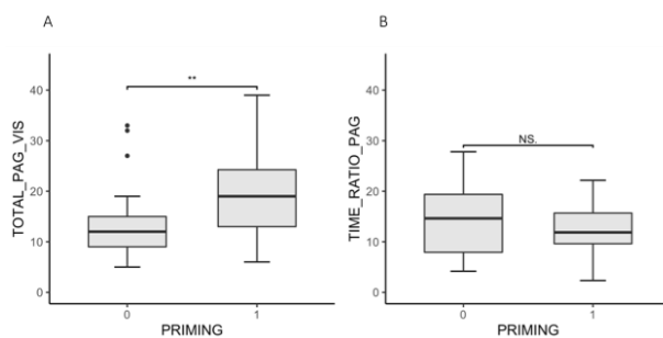
Figure 2. Boxplot for H_1 and H_2 (Mann-Whitney test)
